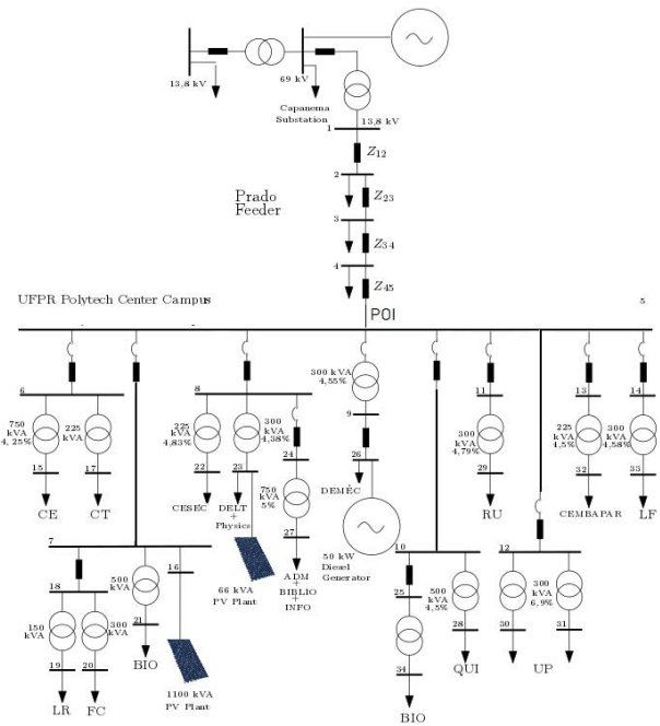
Fig. 1. Single-line diagram of the UFPR Campus Microgrid.
